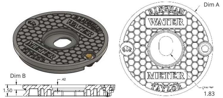
Thru-Hole Lid (Fits Neptune Transmitter)
